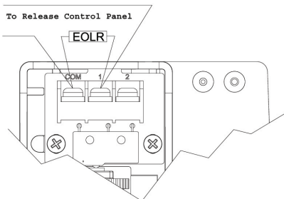
Figure 2 - Alarm Pressure Switch Wiring (Alarm Pressure Switch should be set to 5 psi)
