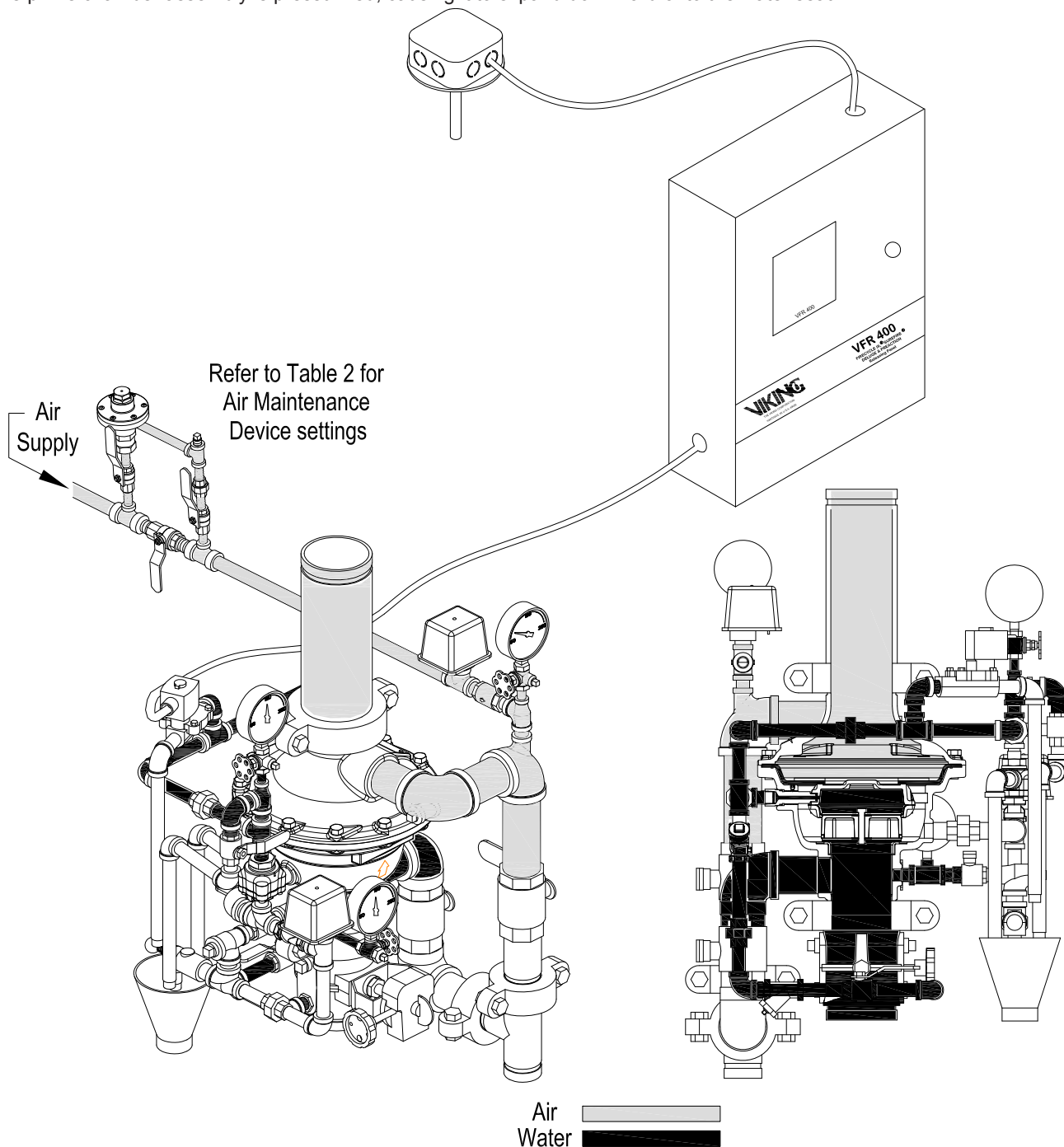
Figure 6 - Set Position
