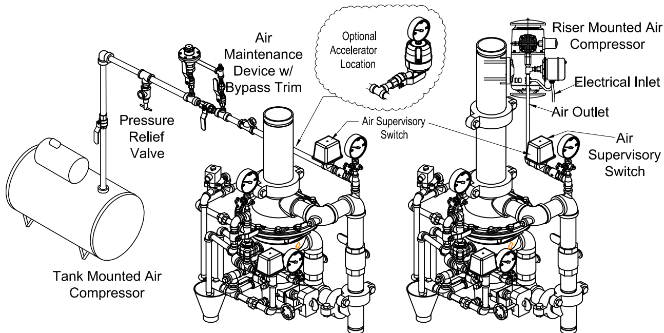
Tank Mounted Air Compressor Option
