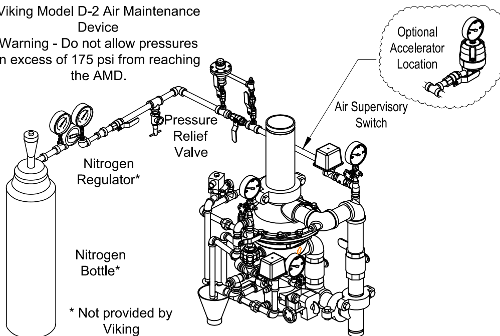
Nitrogen Air Supply Option
