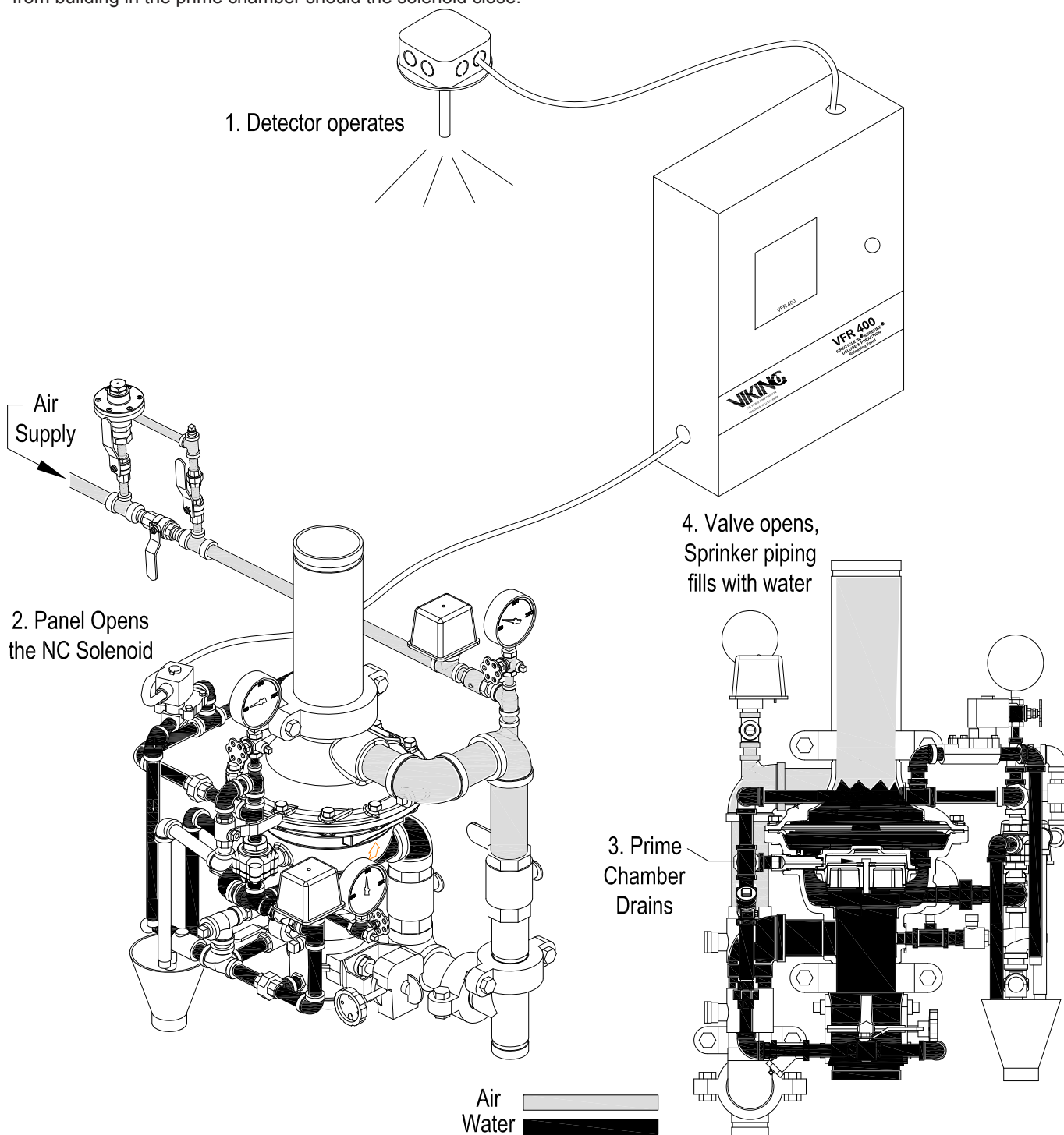
Figure 7a - Activation of Release System - Single Interlock System
