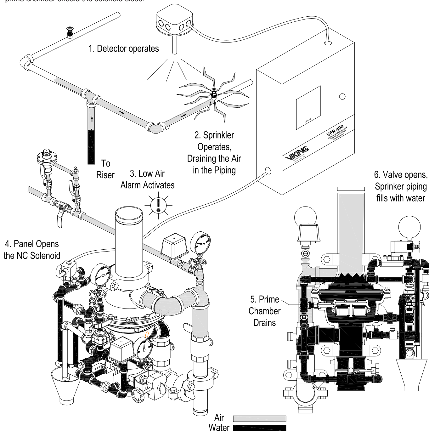
Figure 7b - Fire Condition - Double Interlock System
