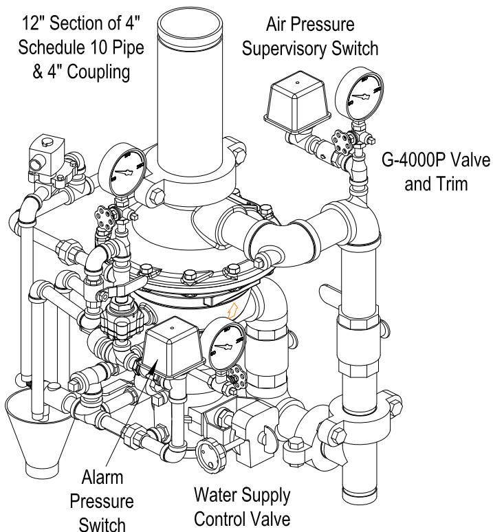
Figure 8 - 15651-1 Assembly
