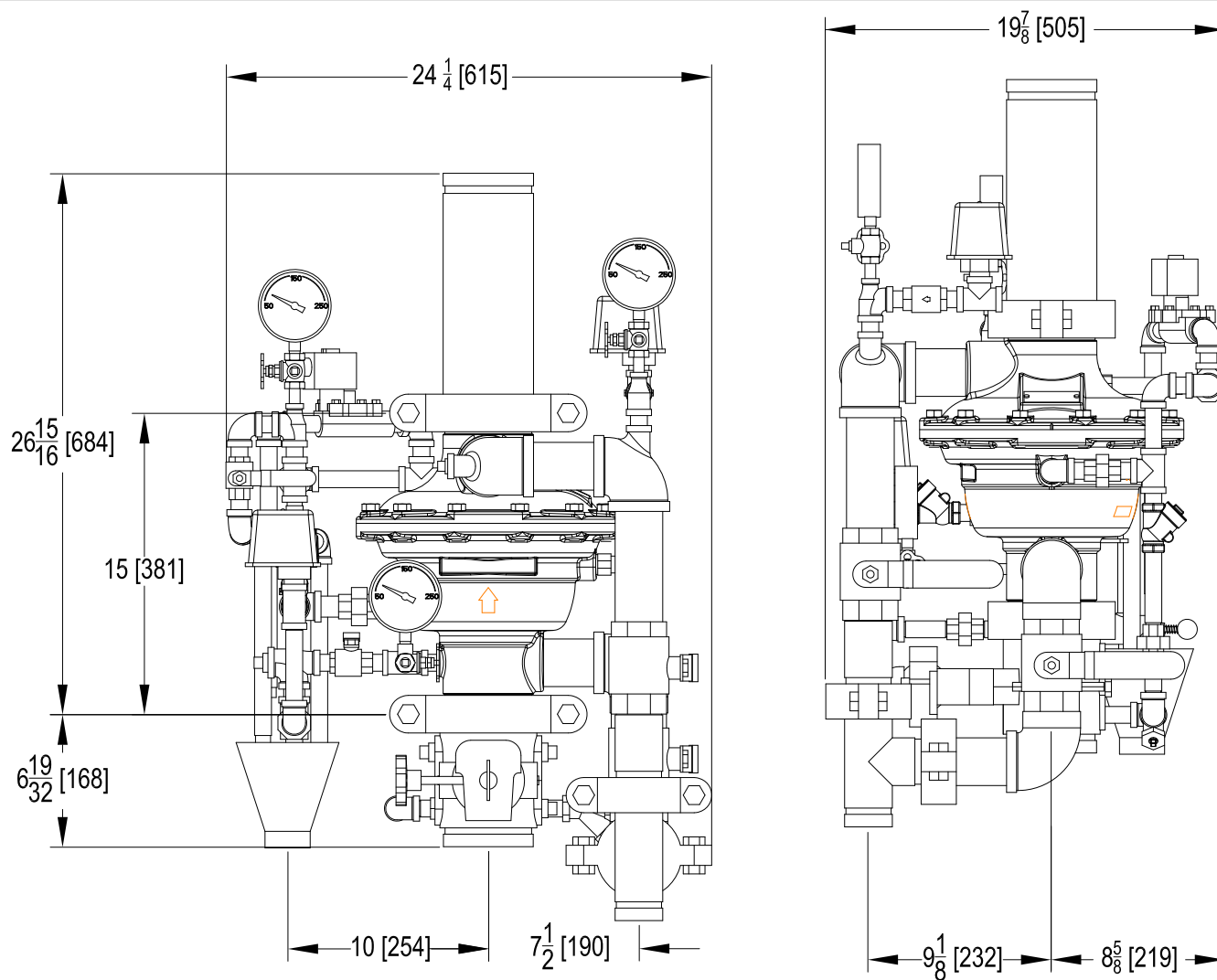
Figure 10 - Installation Dimensions
